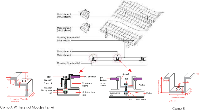
Figure 3: Clamp Details (Units: mm)
