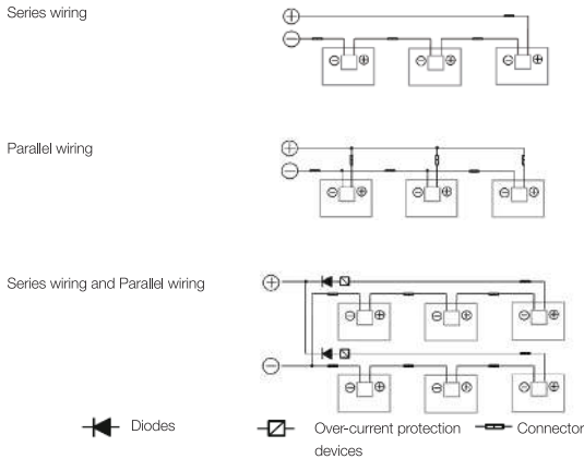
Figure5: Electrical diagrams of series and parallel wiring
