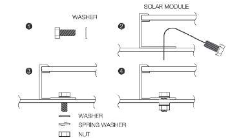
Figure 2 Mounting Details
